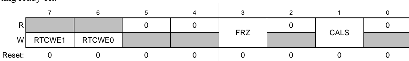
Figure 16-4. RTC Control Register 3(RTCCTL3)
