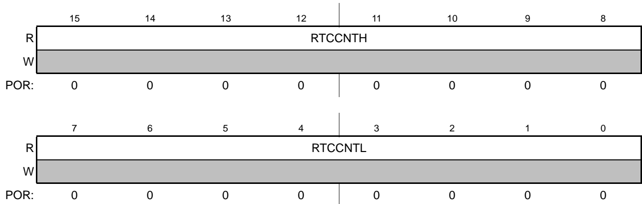
Figure 16-8. RTC Counter Register (RTCCNT)
