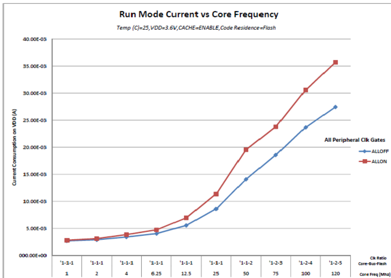
Figure 3. Run mode supply current vs. core frequency
