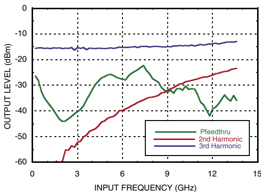
Output Harmonic
