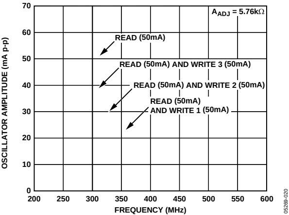
Figure 4. Oscillator Amplitude vs. Frequency
