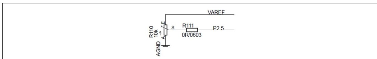
Figure 5 Potentiometer Circuit
