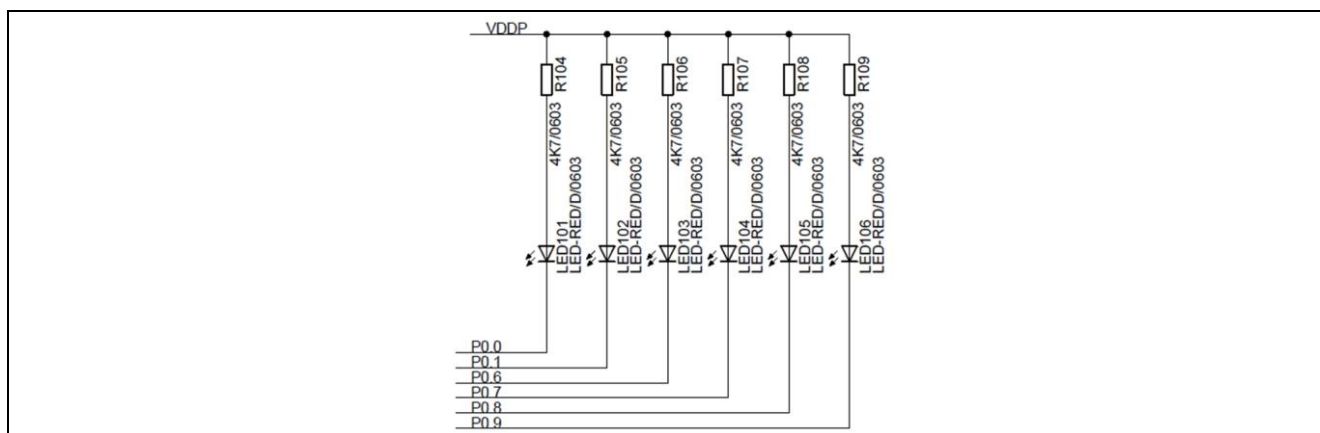
Figure 4 LEDs circuit
