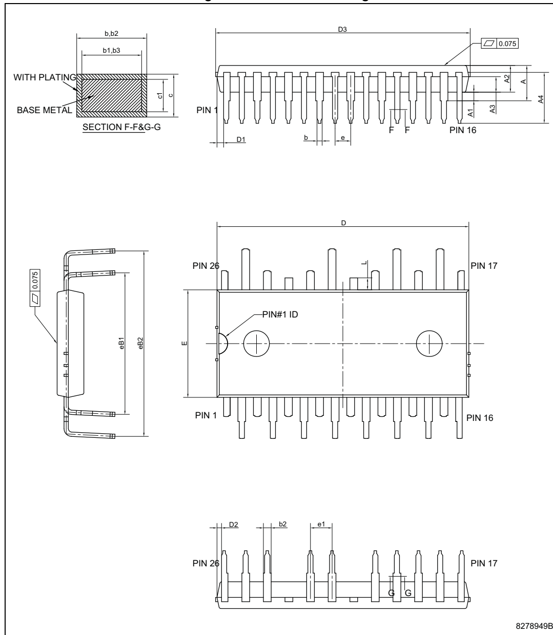
Figure 8. NDIP-26L drawing
