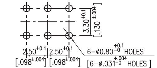
P.C.B. LAYOUT (VIEW FROM THE DIRECTION A)
