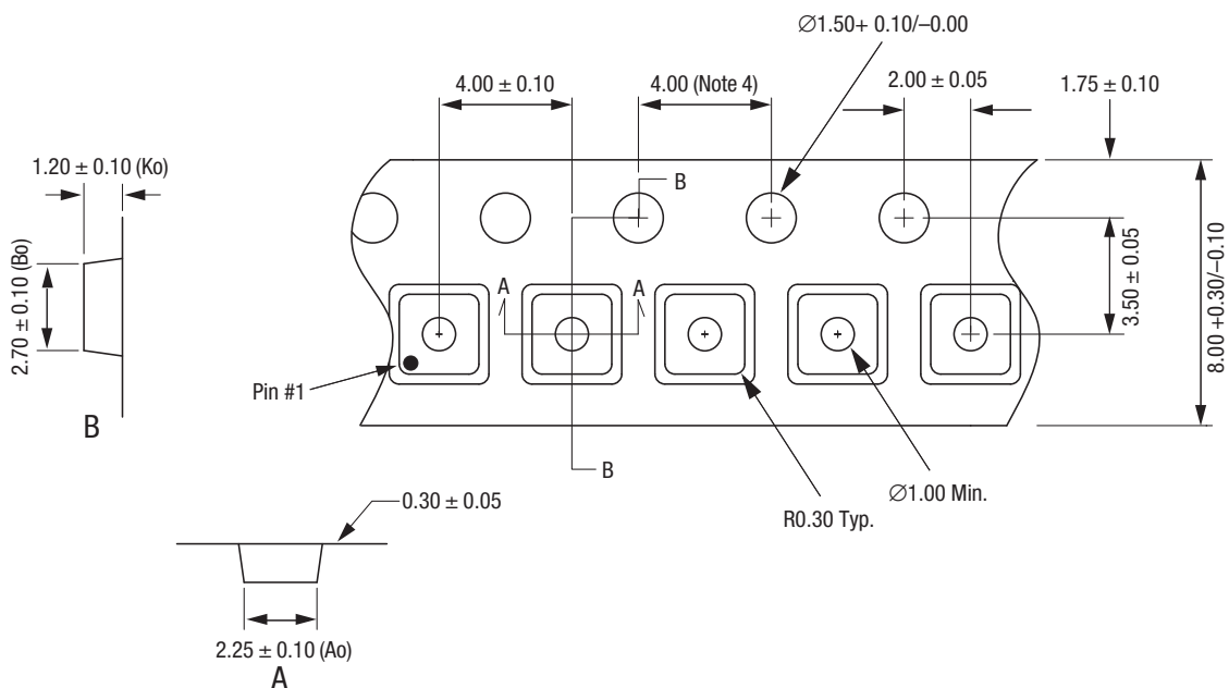
Figure 7. AS179-92LF 6-Pin SC-70 Package Dimensions
