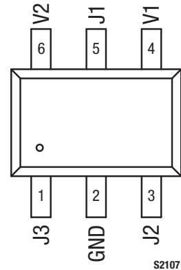
Figure 2. AS179-92LF Pinout –6-Pin SC-70 (Top View)
