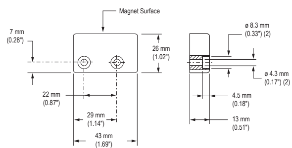
Figure 16. SI-MAG2MM Magnet
