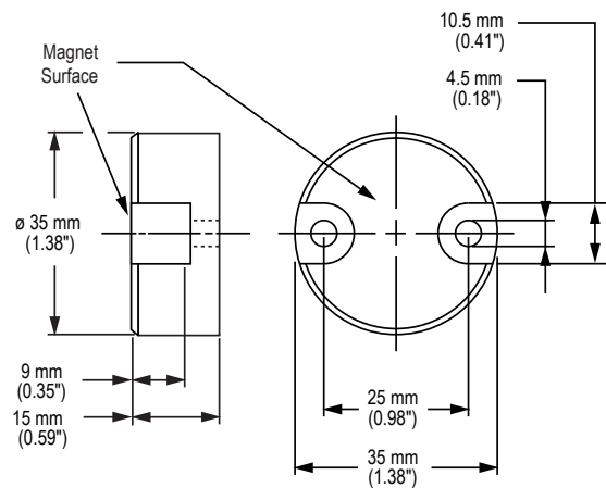
Figure 18. SI-MAG3MM Magnet
