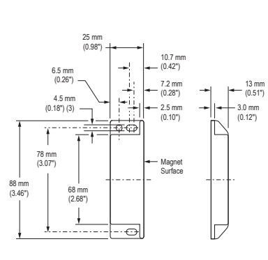
Figure 14. SI-MAG1MM/MM90/MMHF Magnet
