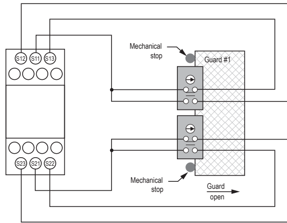
Figure 3. Wiring to two positive-opening safety interlock switches
