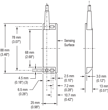
Figure 13. SI-MAG1SMCO Sensor
