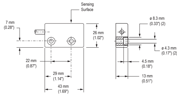
Figure 15. SI-MAG2SM Sensor
