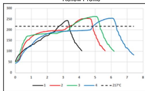
Reflow Profile
