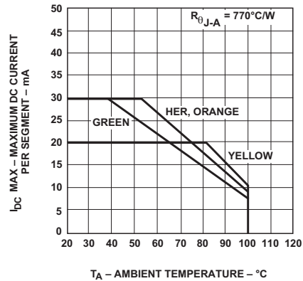
Figure 9. Maximum Allowable DC Current per Segment as a Function of Ambient Temperature.
