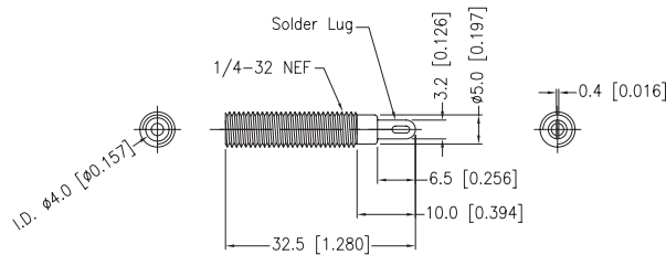
THREADED BODY
