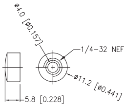
INSULATED HEAD
