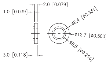
INSULATED WASHER
