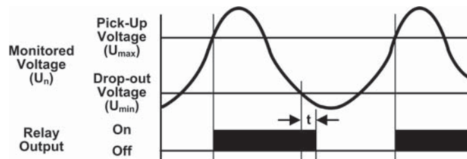
Adjustable Pick-Up, Fixed & Drop-Out Settings* Adjustable Time Delay on Drop-out at 0.1-10 Seconds
