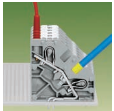
Solid wires and fine-stranded wires with ferrules can be simply pushed in Testing with test plug Ø 2 mm/0.079 in
