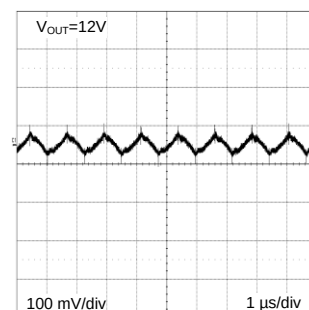
Output Ripple
