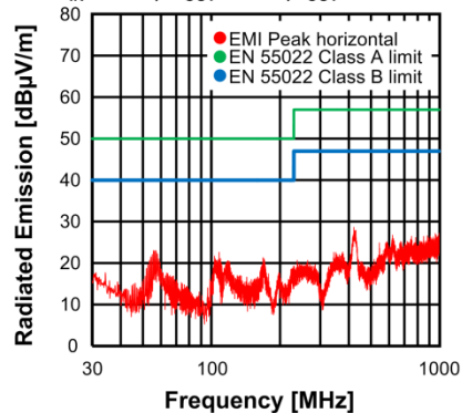
Radiated EMI according to EN55022 (CISPR-22); Measured on Evaluation Board at 3m antenna distance; V_{IN} = 24V ; V_{OUT} = 12V ; I_{OUT} = 1.5A
