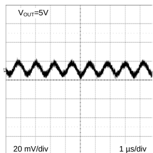
Output Ripple
