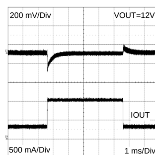
Load Transient Response V_{IN} = 24V V_{OUT} = 12V Load Step from 30% to 70%
