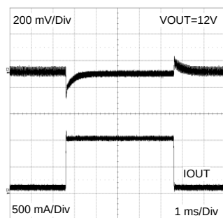
Load Transient Response V_{IN} = 24V V_{OUT} = 12V Load Step from 10% to 70%
