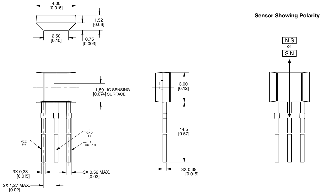
Figure 6. SM451R and SM453R Sensor IC Mounting Dimensions (For reference only. mm/[in].)
