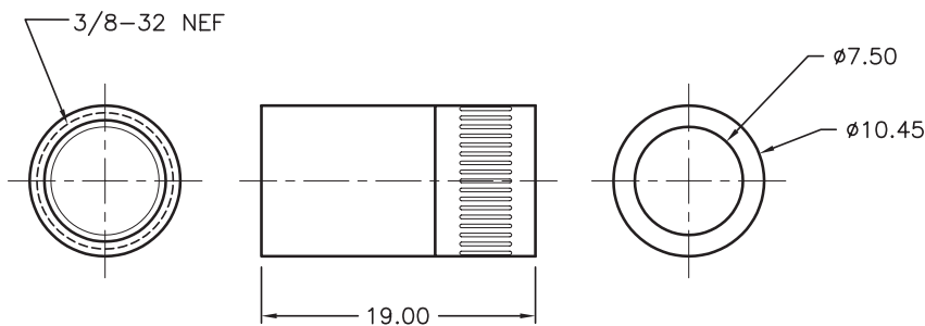
Handle
