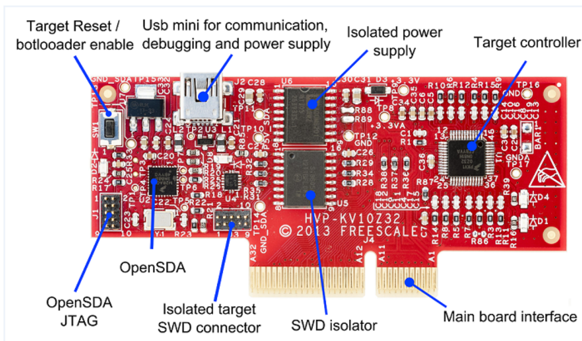
Figure 2. HVP-KV10Z32 controller card description
