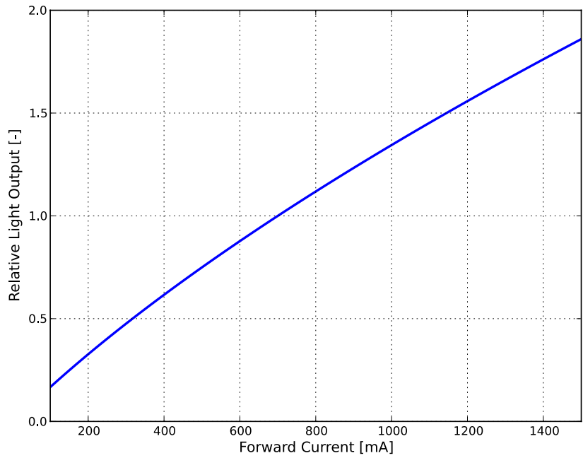
Figure 2b: Typical normalized light output vs. forward current for LUXEON TX, T j =85°C.
