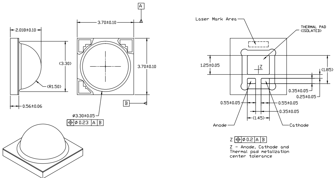
Figure 8: Mechanical dimensions for LUXEON TX.
