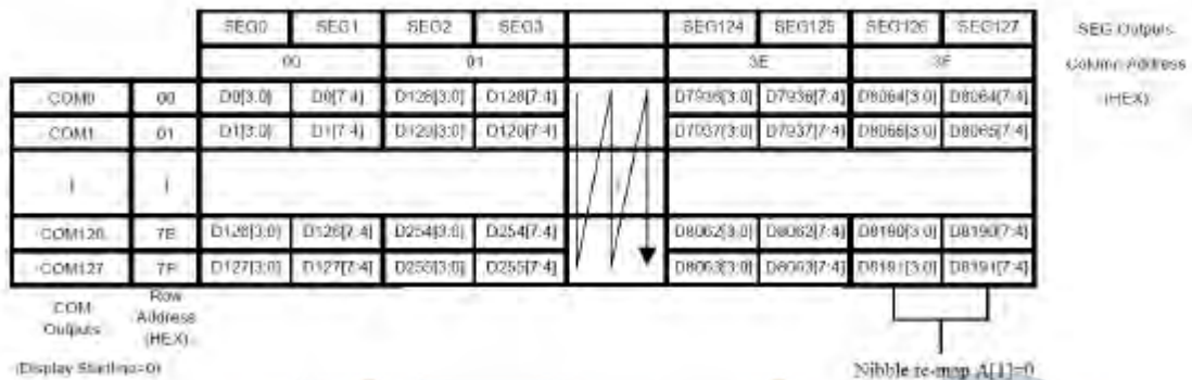
GDDRAM address map 2
