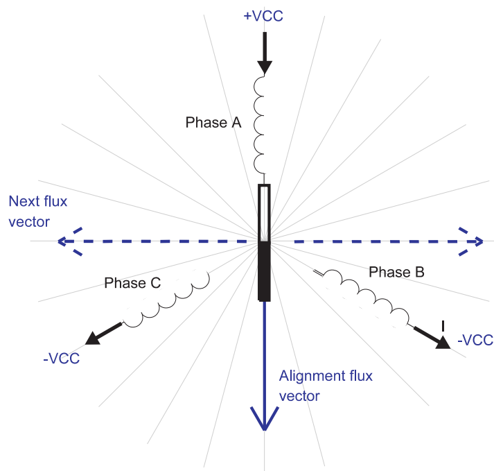
Figure 2-6. Rotor Alignment
