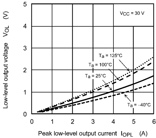
Fig. 12.2.9 V_{OL} - I_{OPL}
