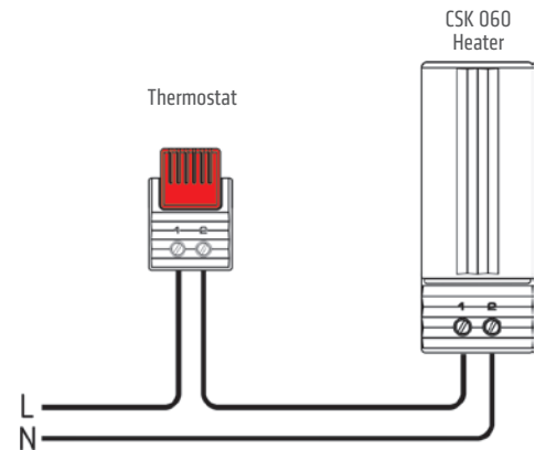
Wiring example
