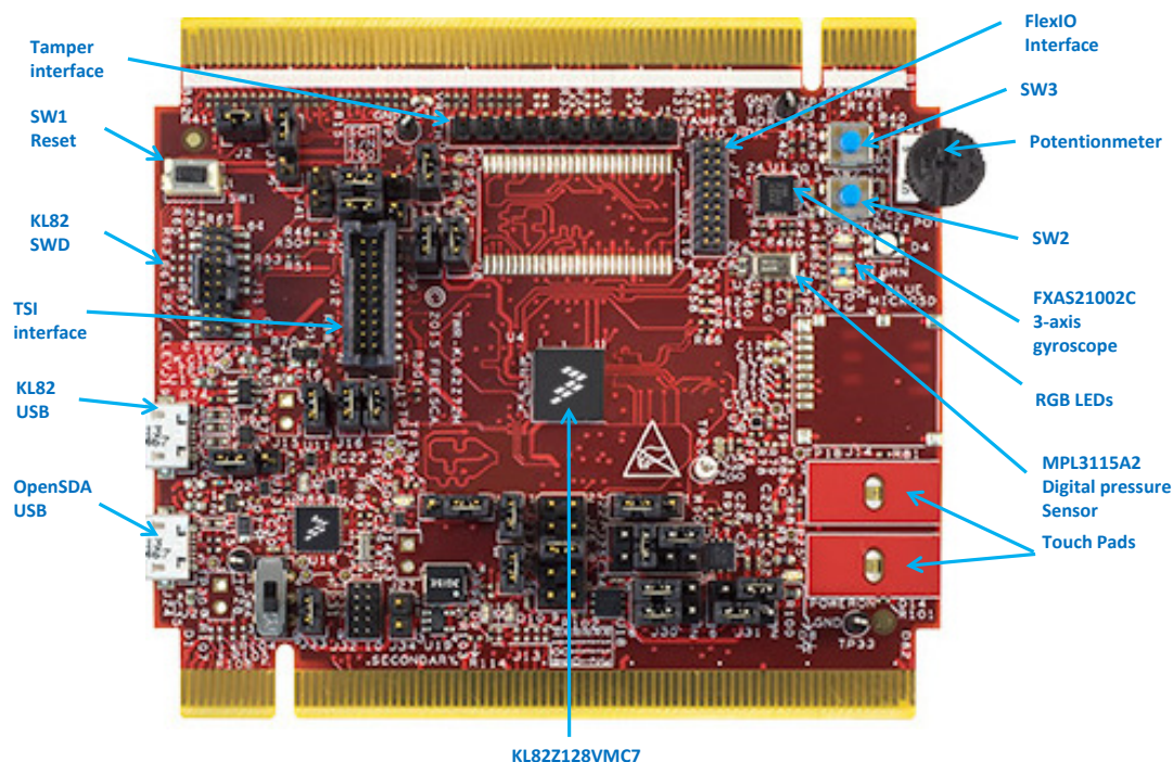
Figure 1. Front side of TWR-KL82Z72M module
