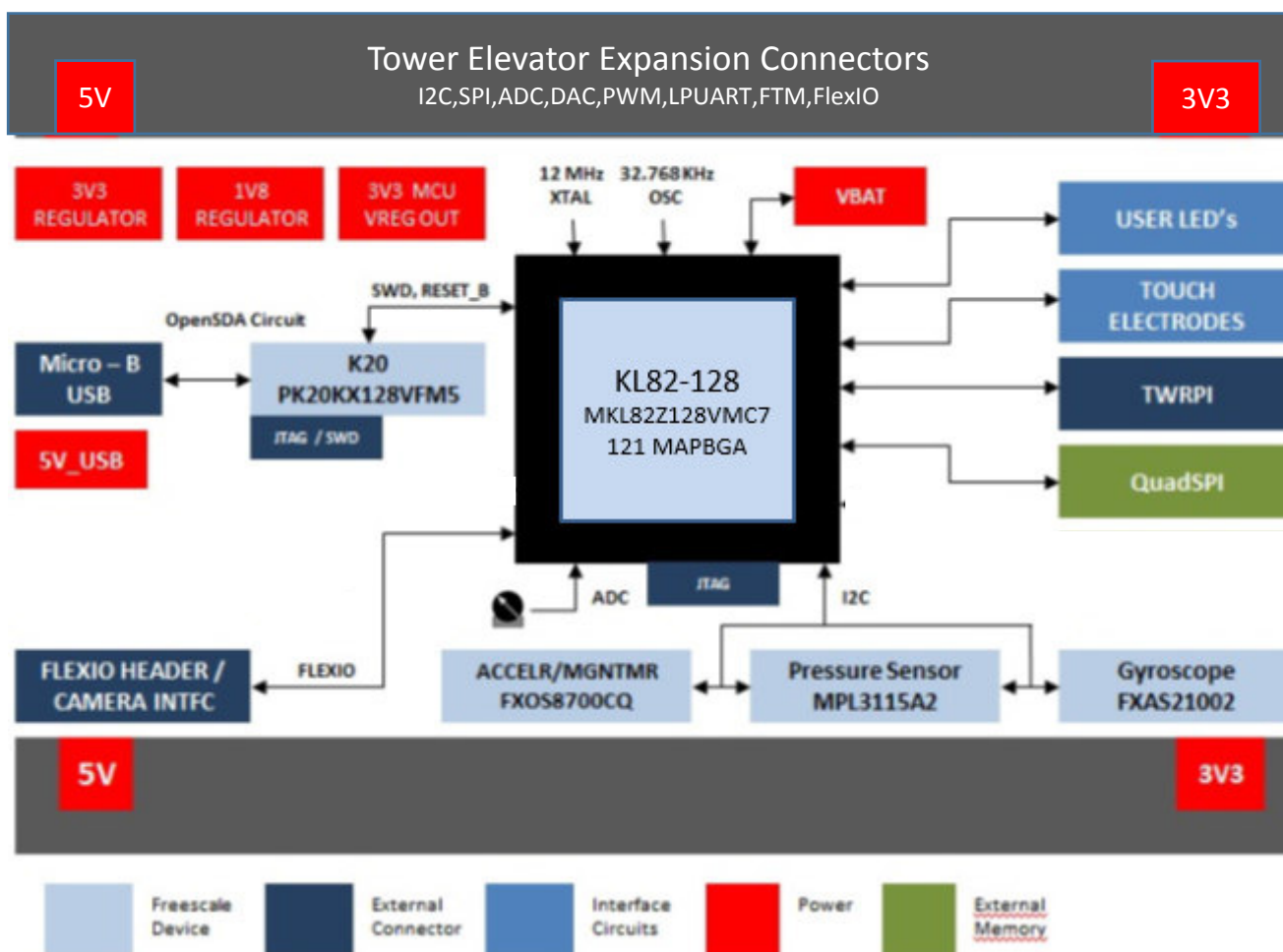
Figure 3. TWR-KL82Z72M block diagram
