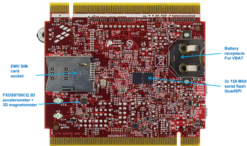
Figure 2. Back side of TWR-KL82Z72M module
