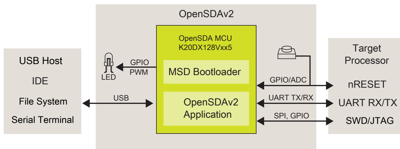
Figure 5. OpenSDAv2 high-level block diagram
