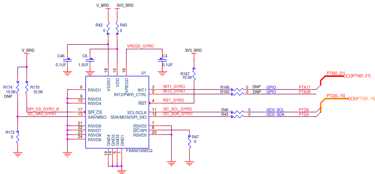
Figure 7. Gyroscope sensor connection
