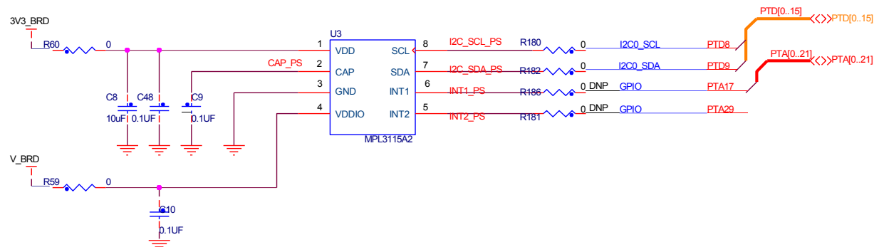
Figure 8. Pressure sensor connection
