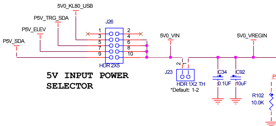
Figure 4. TWR-KL82Z72M power supply
