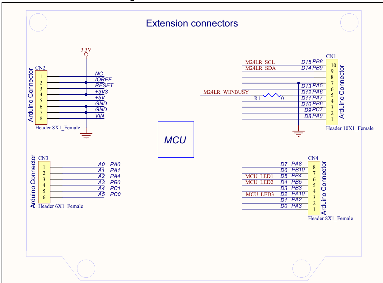
Figure 4. STM32 Nucleo connectors
