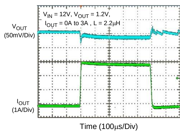
Load Transient
