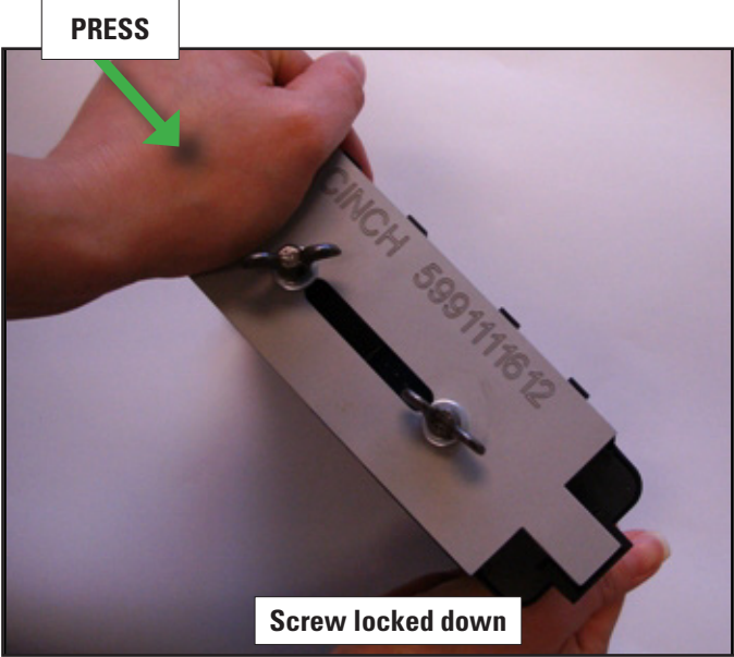
Tighten screw all the way down to release side latch A (audible snap)
