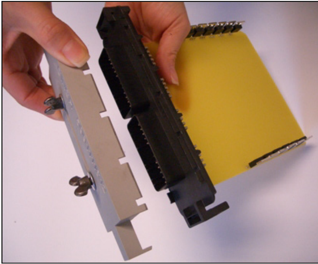
Untighten screws to release the tool from the header
