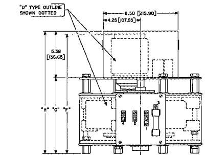
MOTOR DRIVEN
