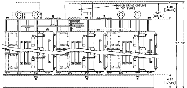
12- TO 27-GANG WYE TYPES
