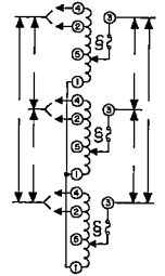
CONNECTION 4
