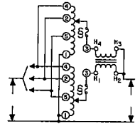
CONNECTION 2
