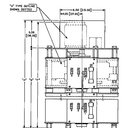
MOTOR DRIVEN
