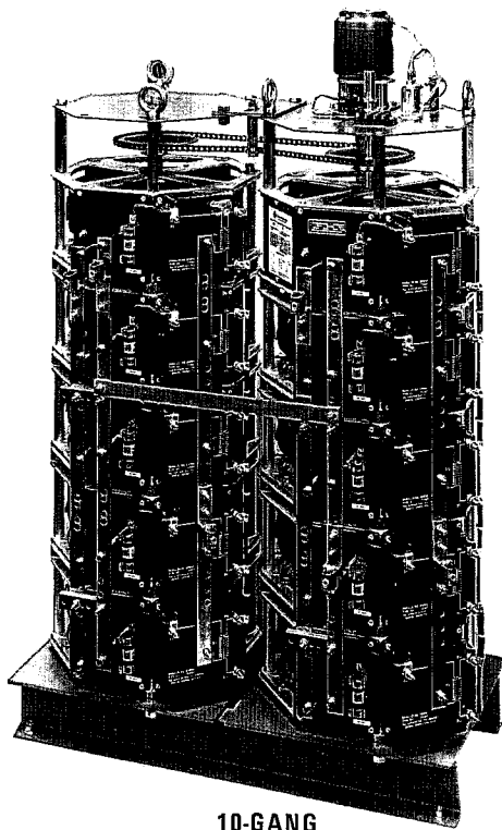
10-GANG MOTOR-DRIVEN ASSEMBLY
