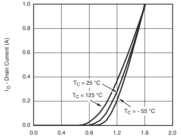
T_C = 25^\circ\text{C} T_C = 125^\circ\text{C} T_C = -55^\circ\text{C} Transfer Characteristics
