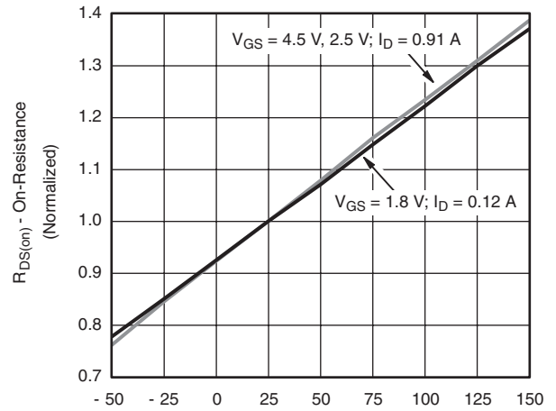
V_{GS} = 4.5\text{ V}, 2.5\text{ V}; I_D = 0.91\text{ A} V_{GS} = 1.8\text{ V}; I_D = 0.12\text{ A} On-Resistance vs. Junction Temperature
