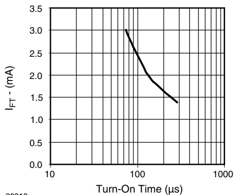
Fig. 8 - I_{FT} (mA) vs. Turn-On Time (μs)
