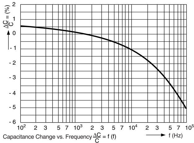
Capacitance Change vs. Frequency ΔC/C = f (f) Capacitance as a function of frequency (typical curve)
