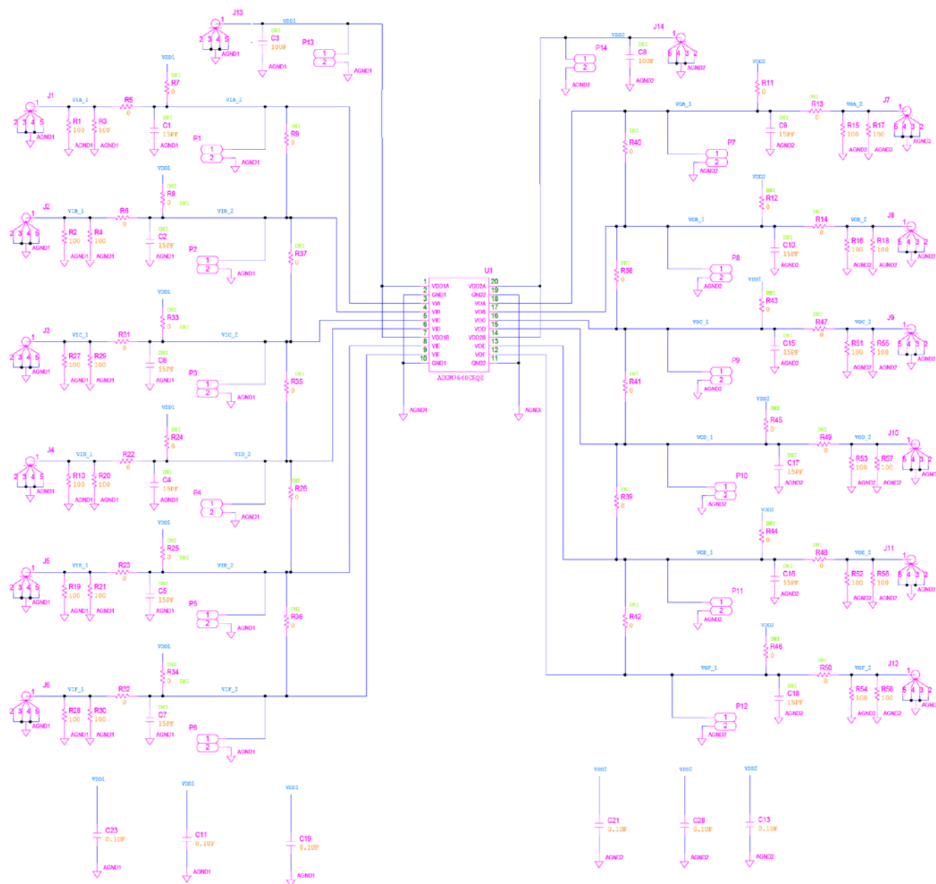
Figure 4. EVAL-ADuM7643EBZ Schematic
