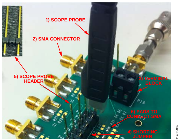
Figure 2. Optional Components
