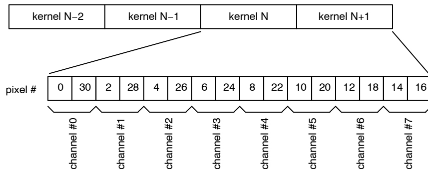
Figure 41. P1-SN/FN: Data Output Order for 8 LVDS Output Channels in Subsampling Mode on a Monochrome Sensor
