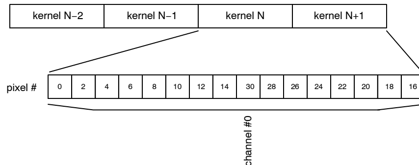
Figure 44. P1,P3-SN/FN: Data Output Order for 1 LVDS Output Channels in Subsampling Mode on a Monochrome Sensor
