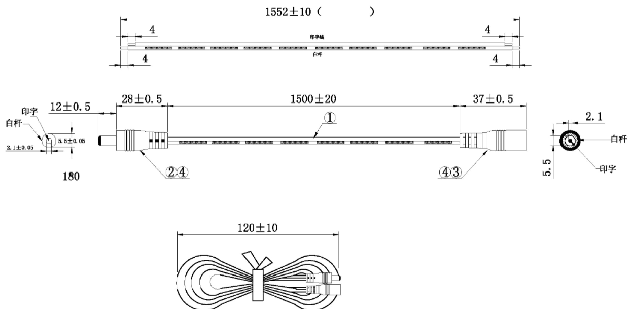
Drawing of CW01903-HD cable
