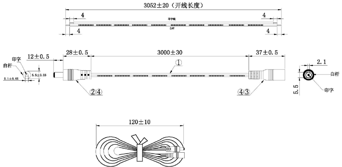
Drawing of CW01905-HD cable
