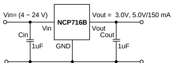
Figure 1. Typical Application Schematic
