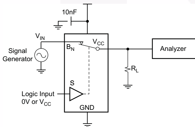
Figure 14. Harmonic Distortion
