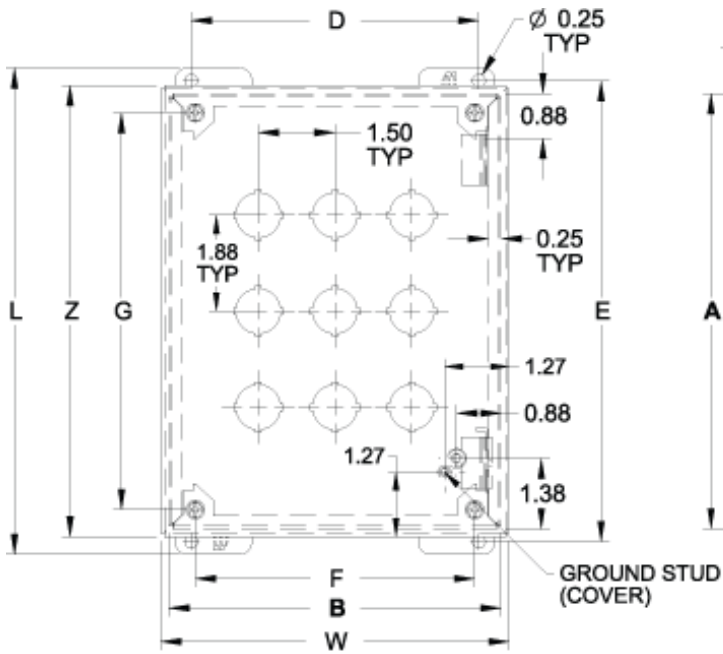
Front View Body Type MPB6 through MPB12 (Hinged)
