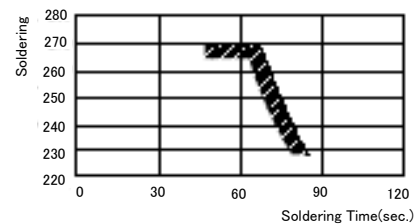
[Allowable Soldering Temperature and Time]
