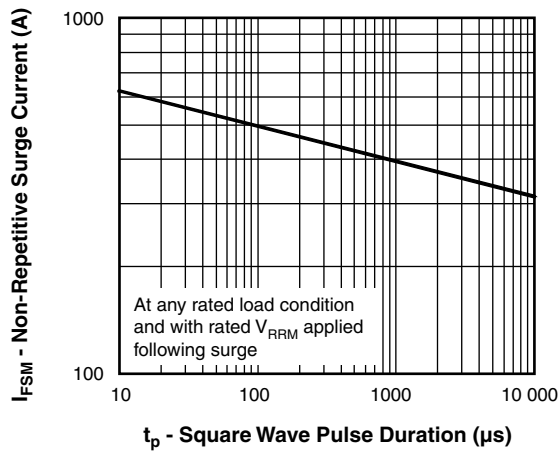
Fig. 7 - Maximum Non-Replicative Surge Current
