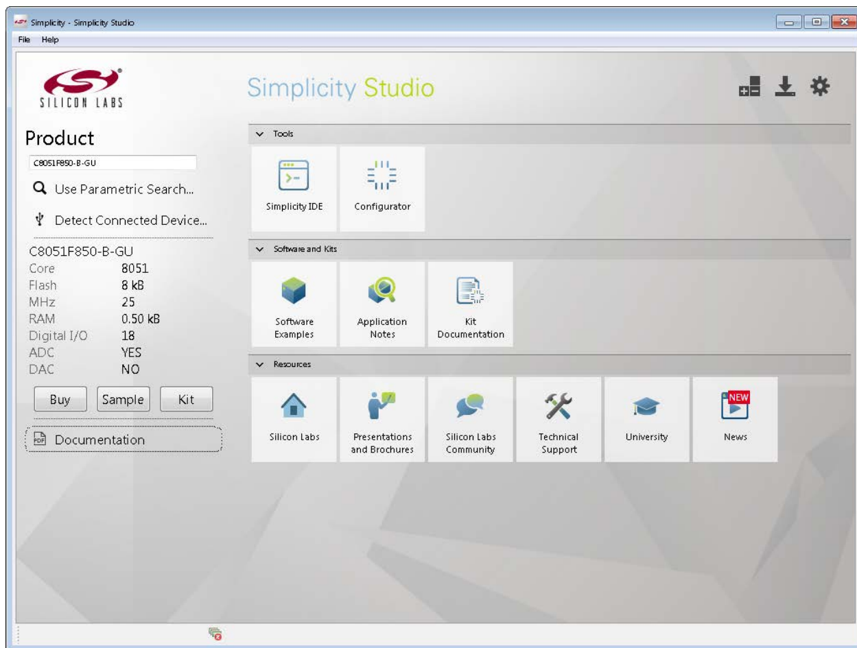
Figure 4. Simplicity Studio
