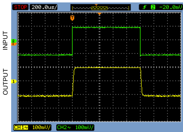
Small-Signal Transient Response V_{DD} = 5.5\text{V} , V_{SS} = \text{GND} , R_{LOAD} = 100\text{k}\Omega , C_{LOAD} = 15\text{pF}
