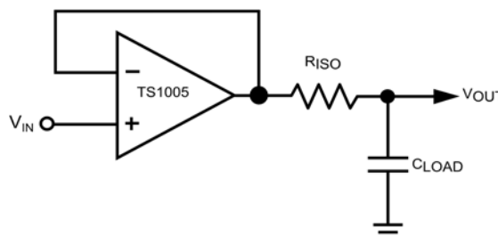
Figure 5: Using an External Resistor to Isolate a C_{LOAD} from the TS1005's Output
