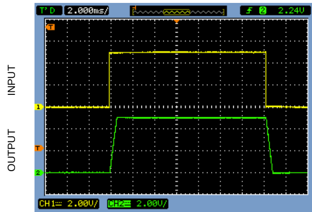
Large-Signal Transient Response V_{DD} = 5.5\text{V} , V_{SS} = \text{GND} , R_{LOAD} = 100\text{k}\Omega , C_{LOAD} = 15\text{pF}
