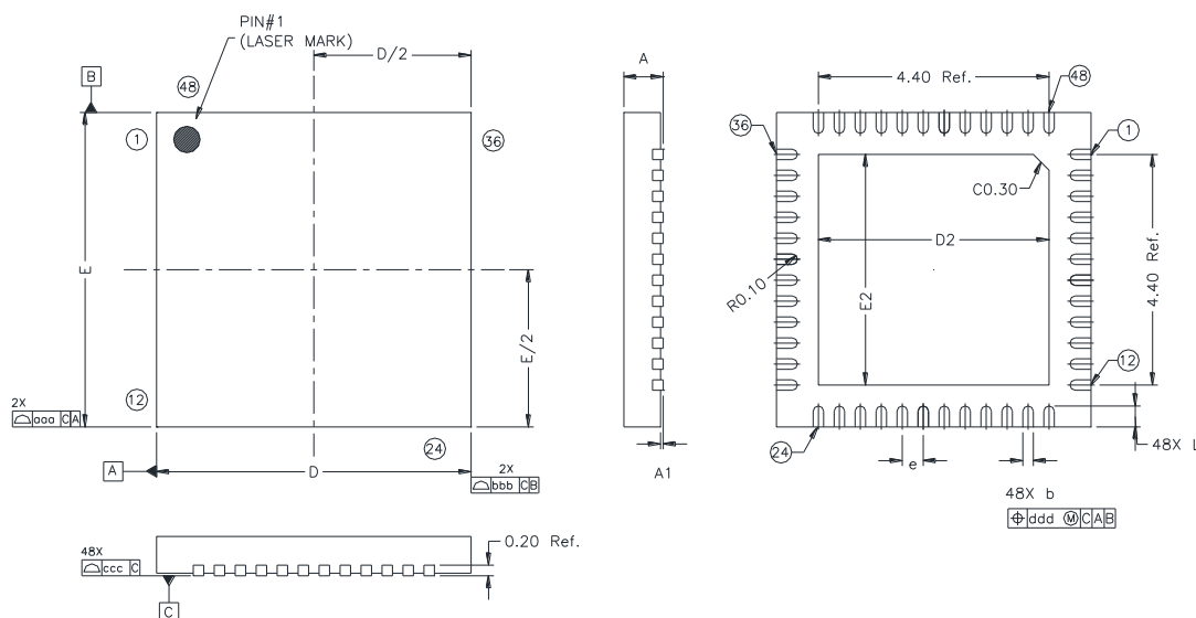
Figure 4. 48-Pin Quad Flat No Lead (QFN) Package
