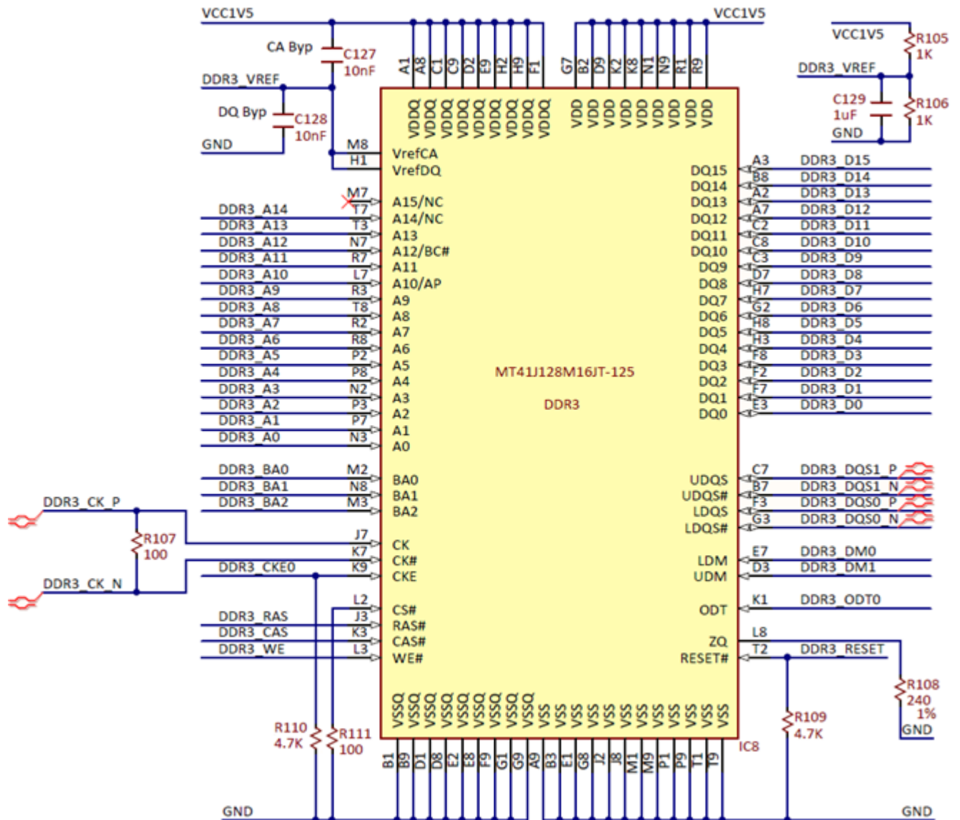
Figure 19. DDR3 memory.
