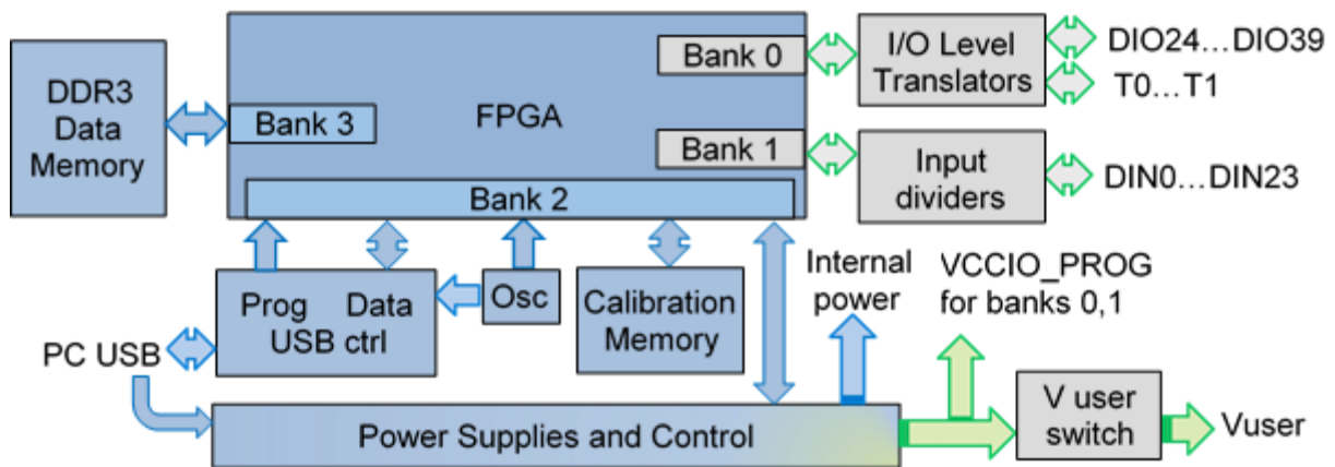
Figure 2. Digital Discovery Hardware block diagram.
