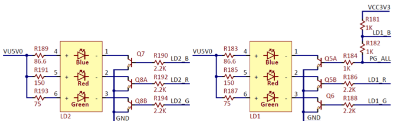
Figure 18. LEDs.
