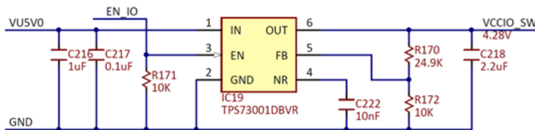
Figure 5. VCCIO_SW supply.
