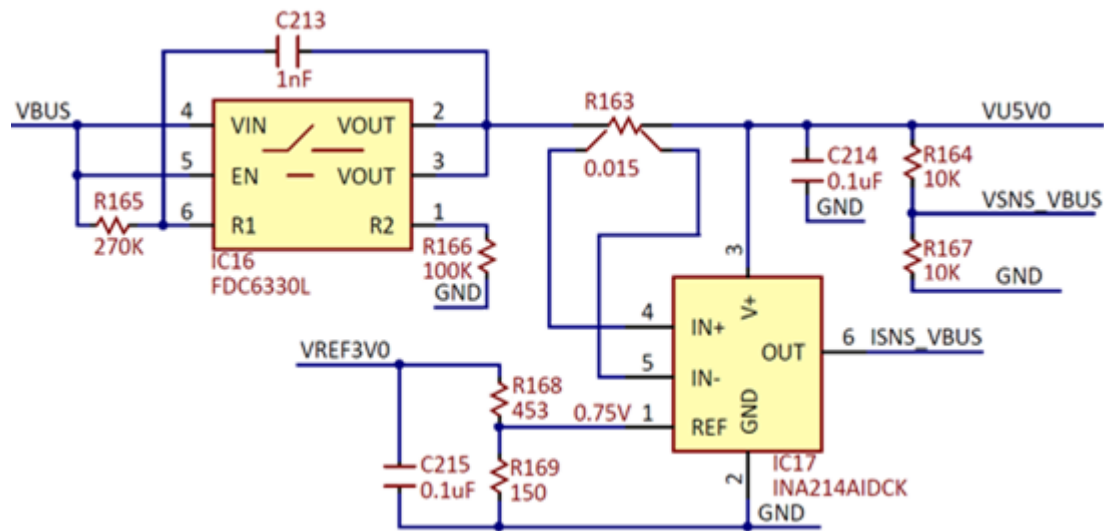
Figure 11 VBUS monitoring.
