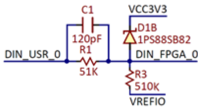
Figure 9. Input Divider.
