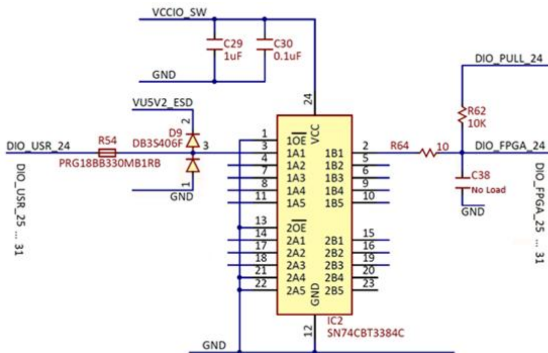
Figure 4. I/O level translator.
