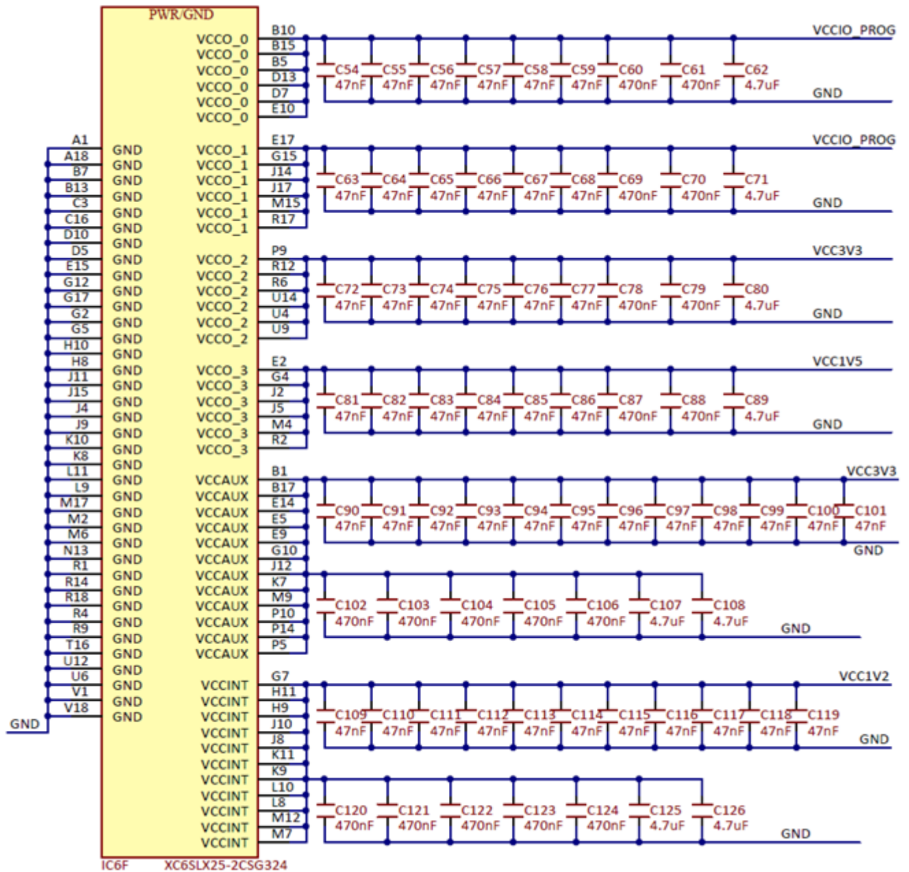
Figure 22. FPGA powering and decoupling.
