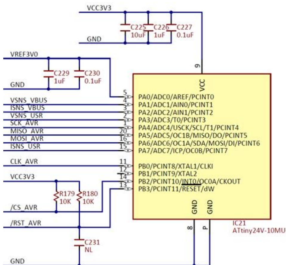
Figure 15. ATtiny microcontroller.
