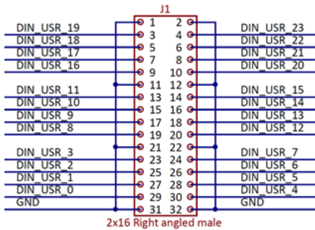
Figure 8. DIN user connector.
