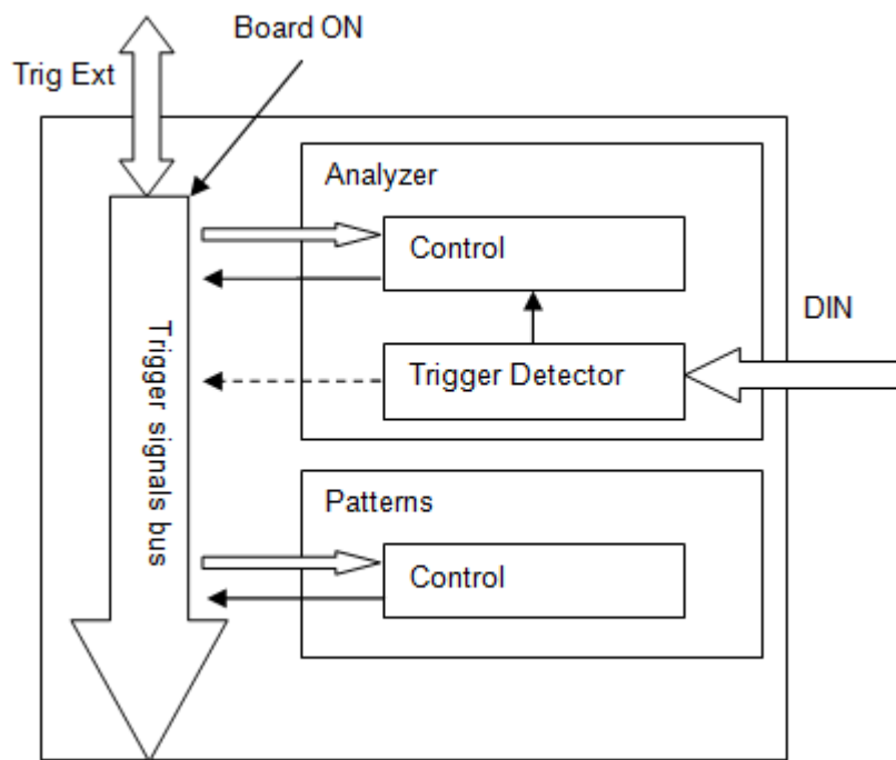
Figure 20. FPGA configuration trigger block diagram.
