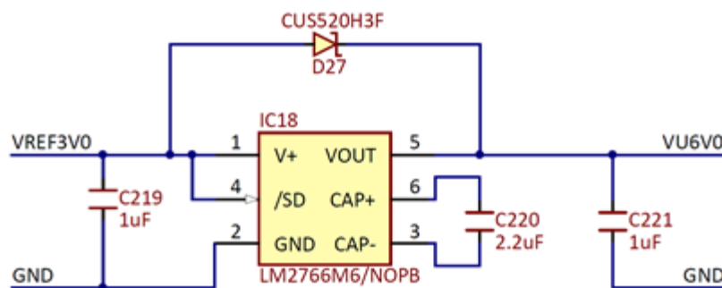
Figure 6. VU6V0 supply.
