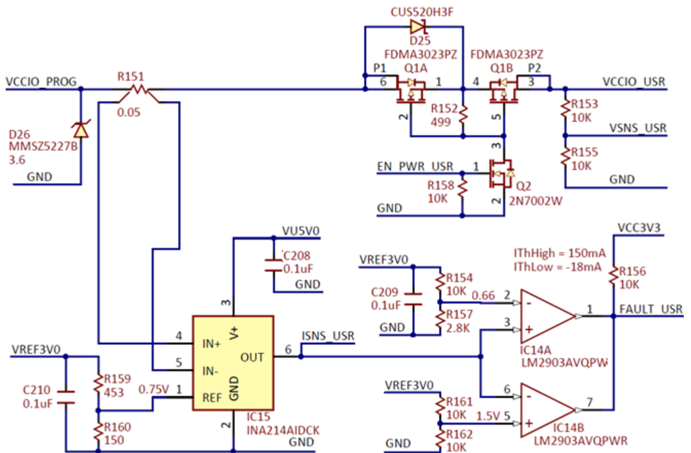
Figure 14. VCCIO_USR protection and switch.
