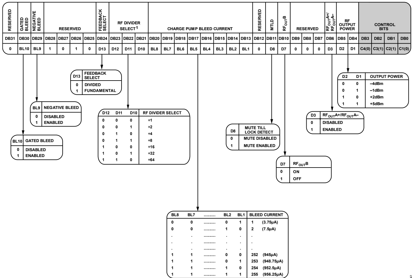
Figure 47. Register 6
