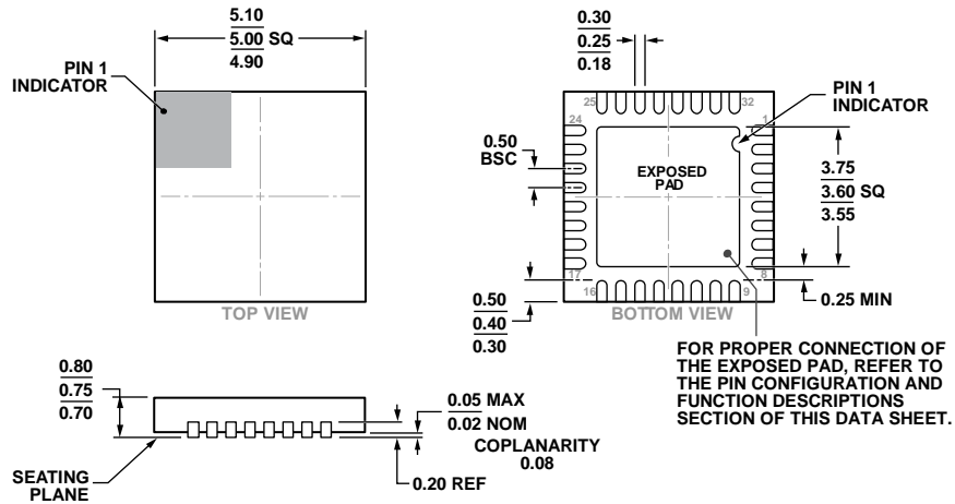
Figure 57. 32-Lead Lead Frame Chip Scale Package [LFCSP_WQ] 5 mm × 5 mm Body, Very, Very Thin Quad (CP-32-12) Dimensions shown in millimeters
