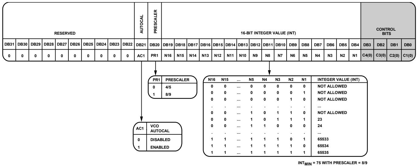
Figure 41. Register 0
