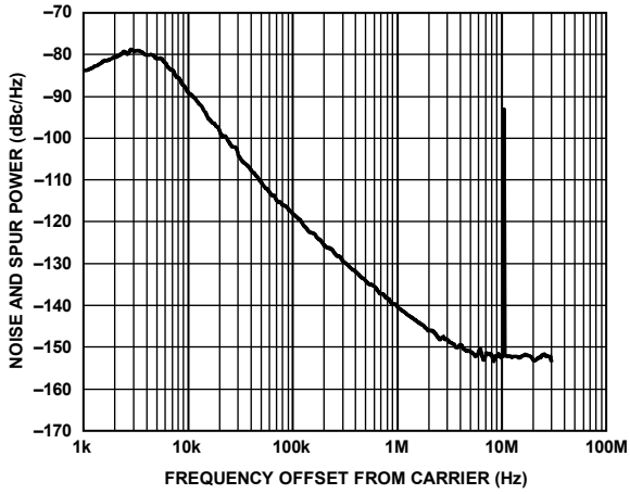
Figure 29. Fractional-N Spur Performance, R_{F_{OUTA+}} = 2.591 GHz, R_{F_{IN}} = 122.88 MHz, f_{PFD} = 61.44 MHz, Output Divide by 2 Selected, Loop Filter Bandwidth = 2 kHz, Channel Spacing = 20 kHz
