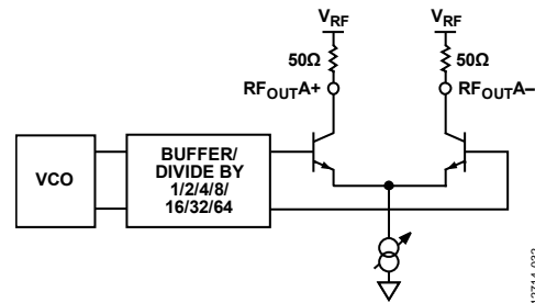
Figure 37. Output Stage
