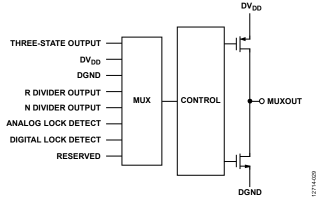
Figure 35. MUXOUT Schematic
