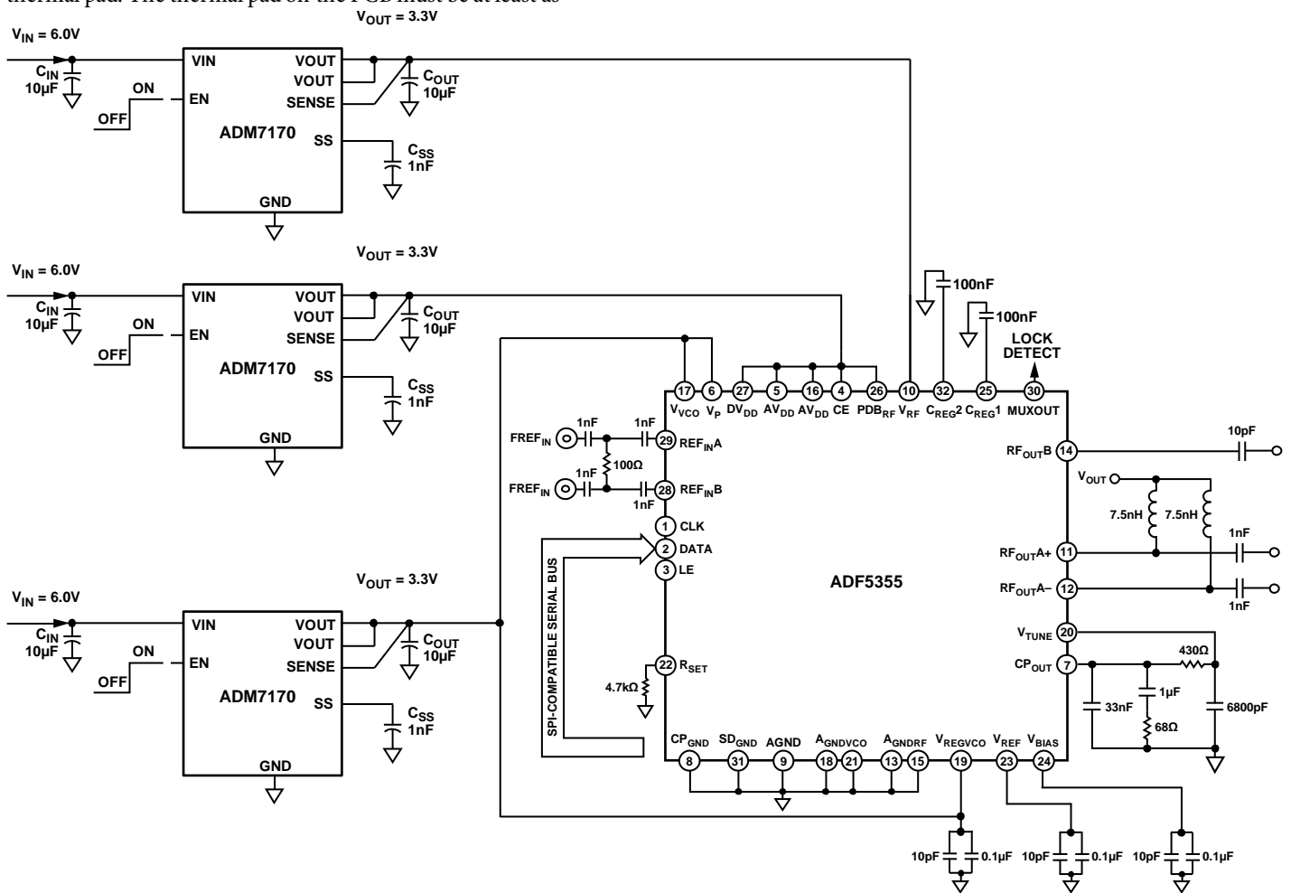
Figure 55. ADF5355 Power Supplies
