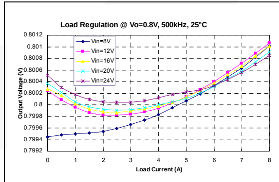
Figure 14. 0.8 V OUT Load Regulation Over V IN vs. Load
