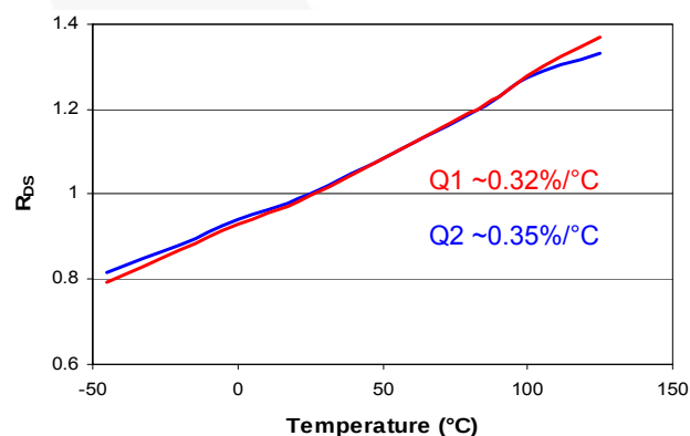
Figure 8. R_{DS} vs. Temperature, Normalized ( V_{CC}=V_{GS}=5V )
