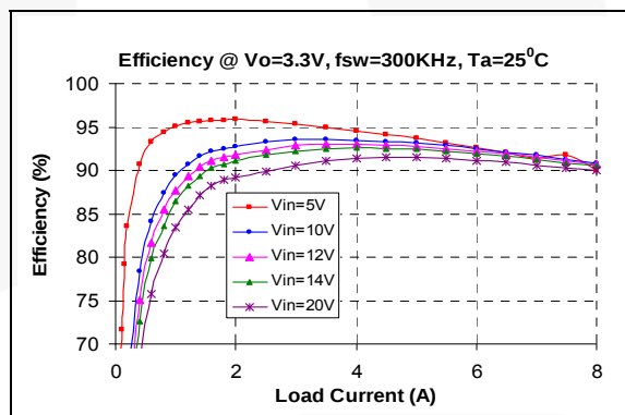
Figure 12. 3.3 V OUT Efficiency Over V IN vs. Load
