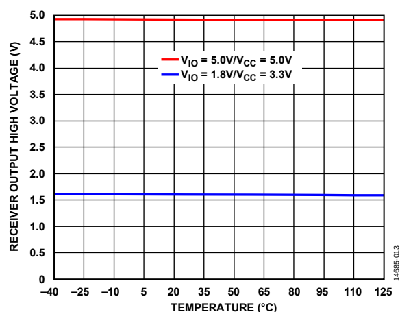
Figure 17. Receiver Output High Voltage vs. Temperature
