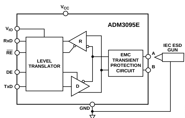
Figure 35. IEC 61000-4-2 ESD Testing Diagram
