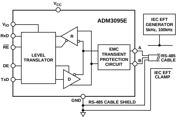
Figure 37. IEC 61000-4-4 EFT Testing Diagram
