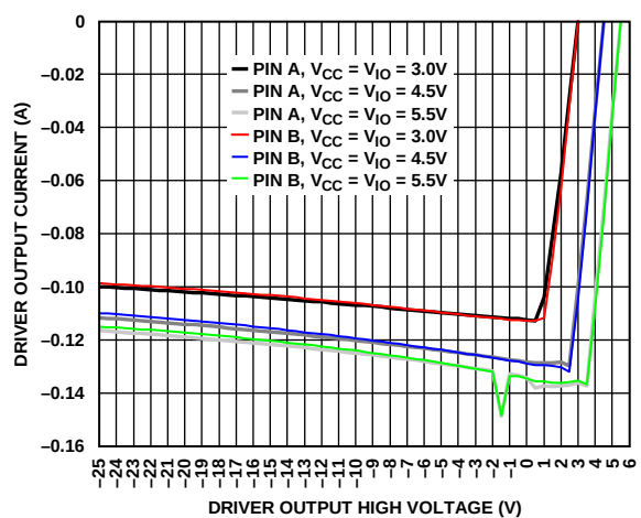
Figure 11. Driver Output Current vs. Driver Output High Voltage
