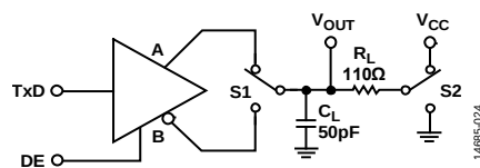
Figure 28. Driver Enable/Disable
