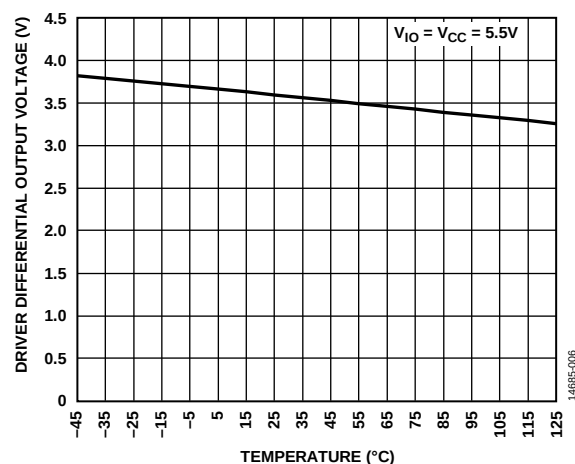
Figure 10. Driver Differential Output Voltage vs. Temperature
