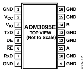
Figure 6. ADM3095E Pin Configuration
