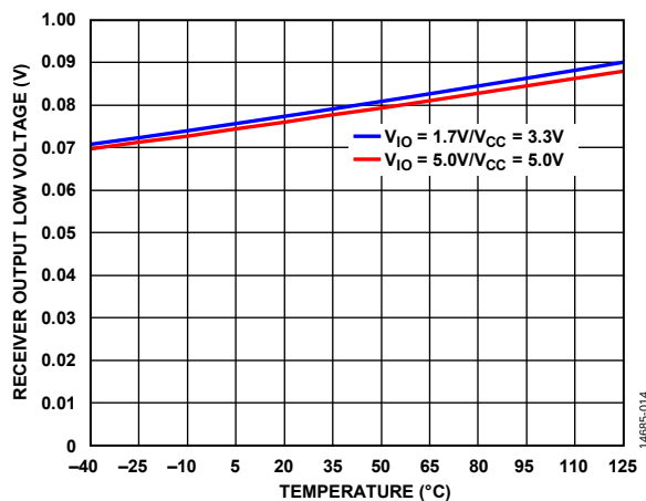
Figure 18. Receiver Output Low Voltage vs. Temperature
