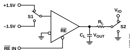
Figure 30. Receiver Enable/Disable
