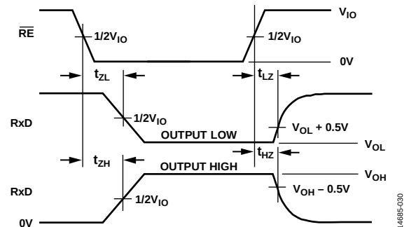
Figure 5. Receiver Enable/Disable Timing Diagram
