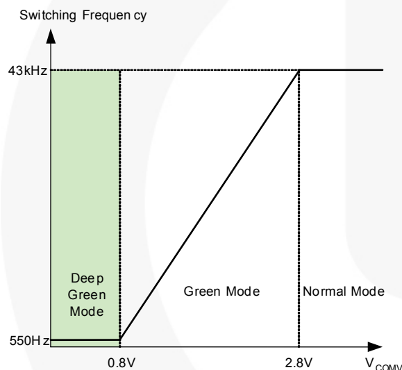
Figure 26. Switching Frequency in Green Mode
