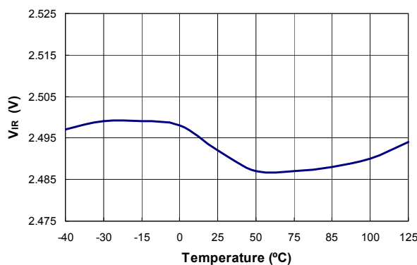
Figure 11. Reference Voltage ( V_{IR} ) vs. Temperature
