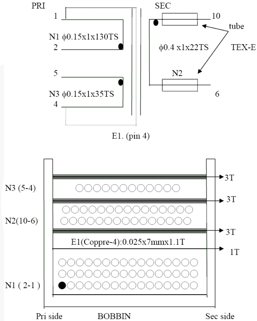
Figure 32. Transformer Diagram
