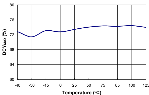
Figure 23. Maximum Duty Cycle ( DCY_{MAX} ) vs. Temperature
