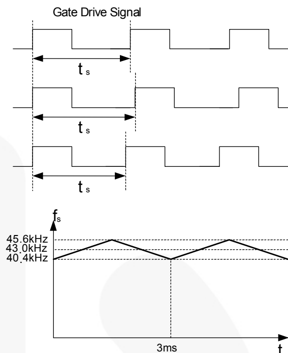
Figure 27. Frequency Hopping
