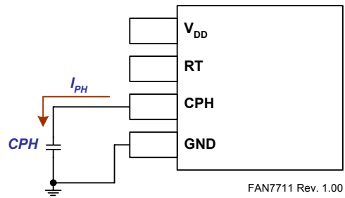
Figure 30. Preheating Timer
