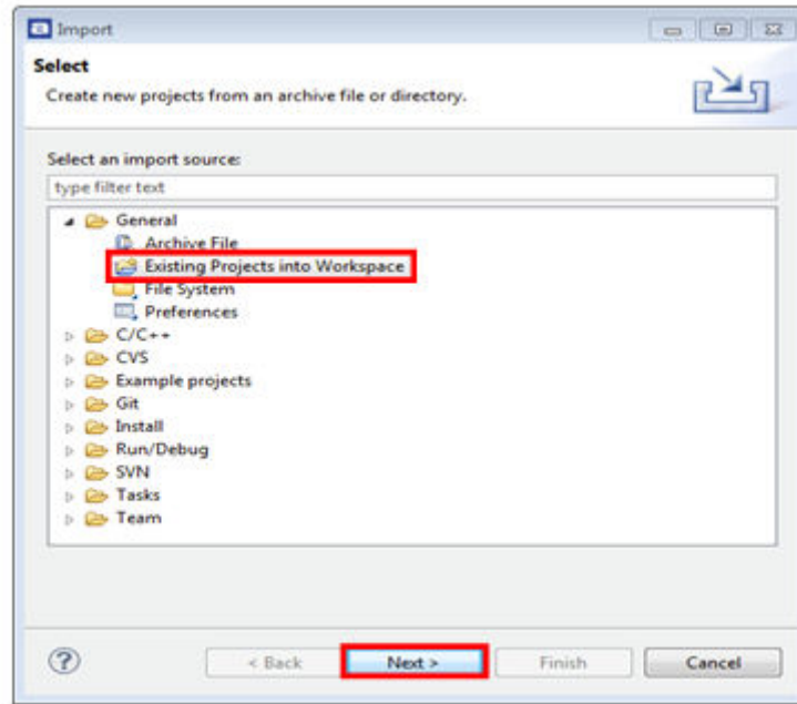
Figure 45. Selection of the correct import type in TrueSTUDIO
