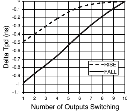
Delta Tpd vs # of Outputs Switching
